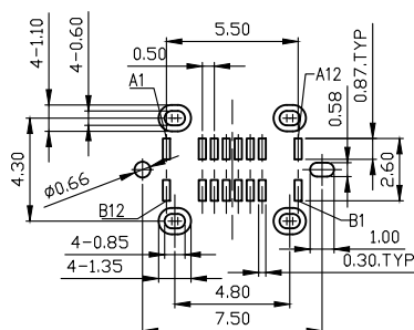
RECOMMENDED PCB LAYOUT TOLERANCE=±0.05 T=1.0
