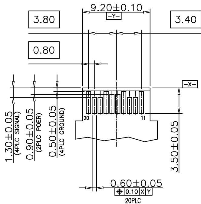
TOP VIEW OF BOARD
