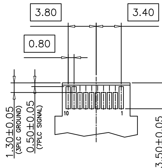
BOTTOM VIEW OF BOARD
