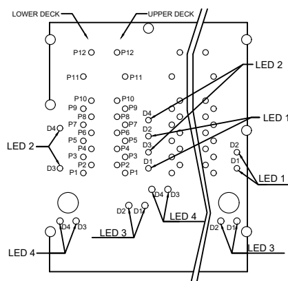
RECOMMENDED PCB LAYOUT (COMPONENT SIDE VIEW)
