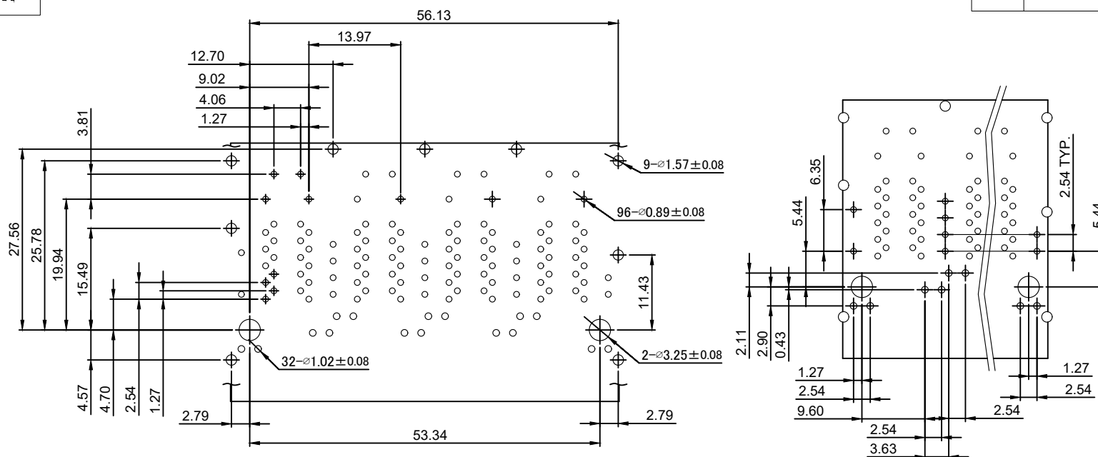
RECOMMENDED PCB LAYOUT (COMPONENT SIDE VIEW)
