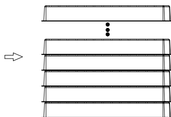
2. TRAYS OVERLAY: (THE NEXT TRAY NEED ROTATE 180 DEGREE AND PUT IT ON PREVIOUS TRAY.) (相邻两个托盘间水平方向成180度摆放)
