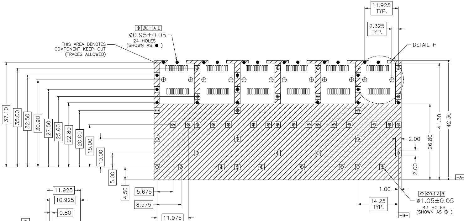
PCB LAYOUT FOR SINGLE SIDE MOUNTING
