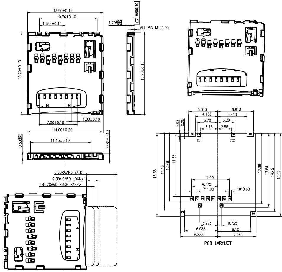
CARD INSERT LARYUOT
