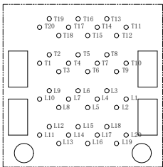
DETAIL D SCALE 2.5:1
