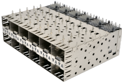
SFP 2X6 Cage+CONN
